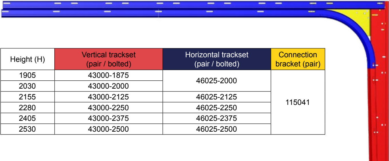
Vertical trackset and horizontal trackset with side connection bracket
