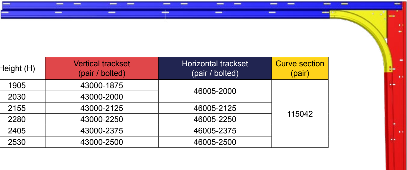
Vertical trackset and horizontal trackset with curve section
